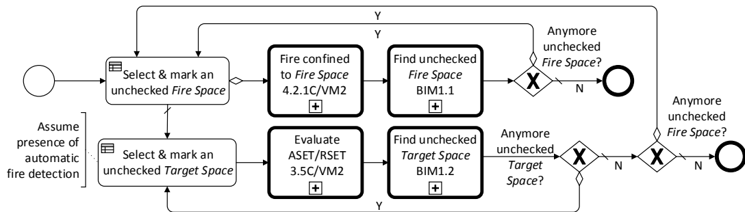
Figure 1: Procedure 4.2C/VM2 – to evaluate UT design scenario
