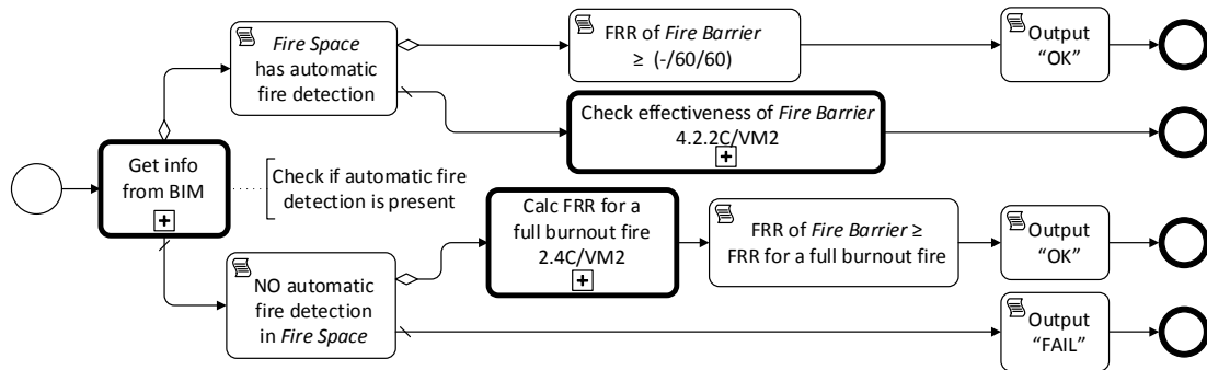
Figure 2: Procedure 4.2.1C/VM2 – to check fire confinement in Fire Space
