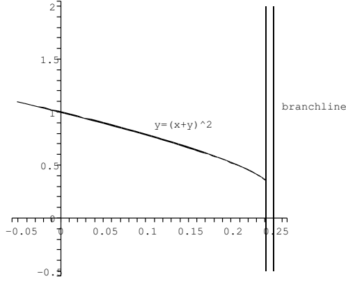
FIG. 7.3. the domain of convergence and the algebraic singularity
