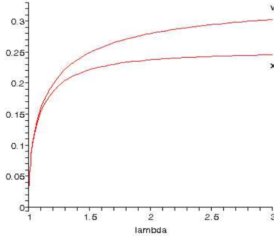
FIG. 4.2. x and v plotted against \lambda
