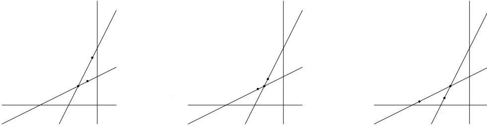
FIG. 4.7. The three possible configurations of critical points
