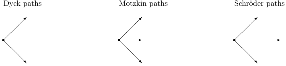
FIG. 7.2. legal steps for three types of paths
