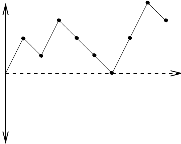
FIG. 7.1. a generalized Dyck path of length nine with E = \{(1, 2), (1, -1)\}
