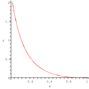
FIG. 4.4. minimal points of \mathcal{V} in the positive real quadrant
