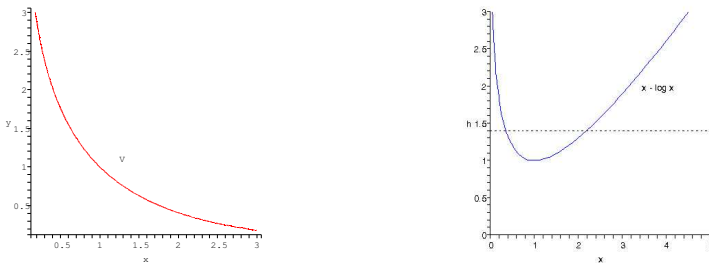
FIG. 4.5. the positive real points of \mathcal{V} and their description by height-pairs
