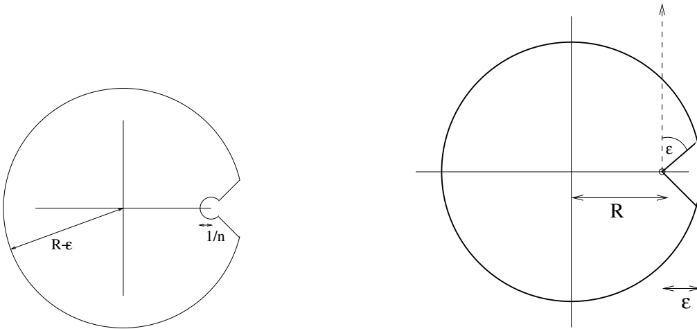
FIG. 2.1. contour for an algebraic singularity and the corresponding region of analyticity
