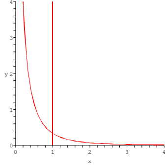
FIG. 4.1. \mathcal{V} in the case d = 3
