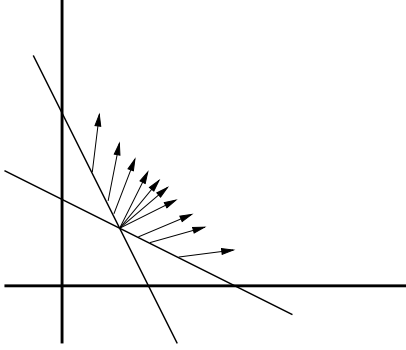
FIG. 3.2. direction \mathbf{L}(\mathbf{z}) for positive real points of \mathcal{V} when 1/F = (3 - x - 2y)(3 - 2x - y)
