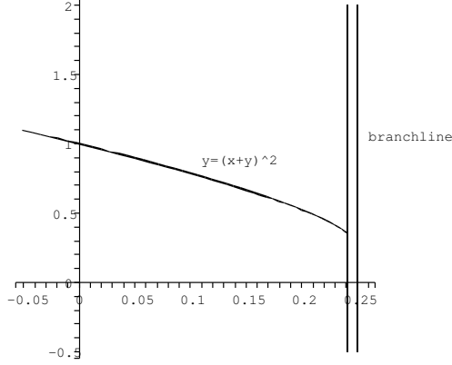
Figure 13: the domain of convergence and the algebraic singularity
