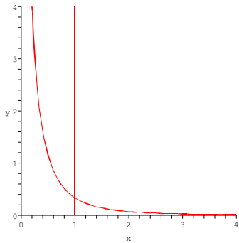
Figure 4: \mathcal{V} in the case d = 3
