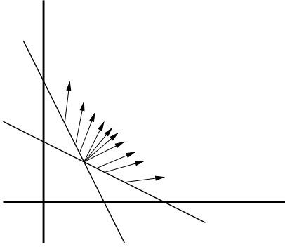
Figure 3: direction \mathbf{L}(\mathbf{z}) for positive real points of \mathcal{V} when 1/F = (3 - x - 2y)(3 - 2x - y)
