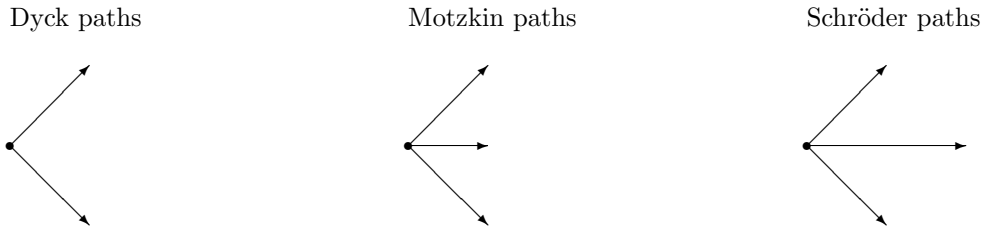
Figure 12: legal steps for three types of paths
