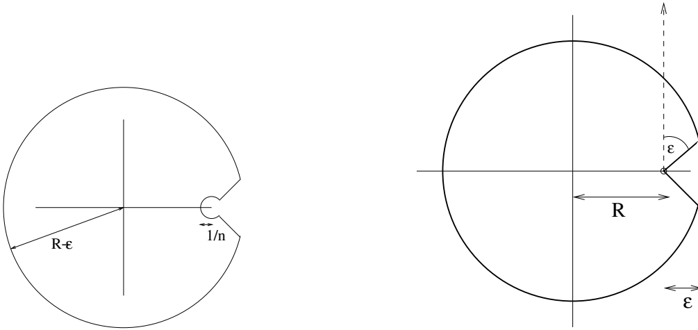
Figure 1: contour for an algebraic singularity and the corresponding region of analyticity
