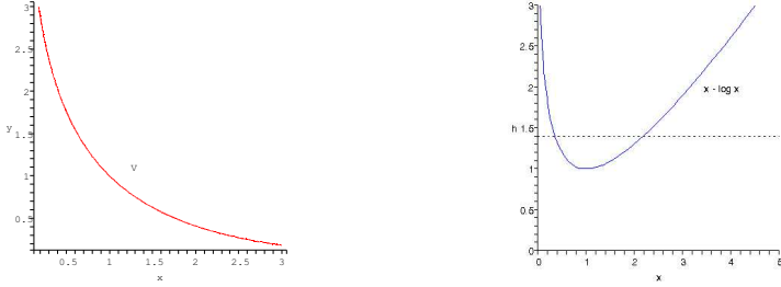
Figure 8: the positive real points of \mathcal{V} and their description by height-pairs
