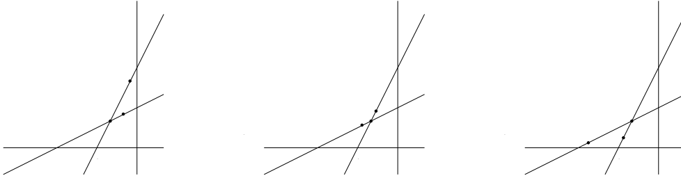
Figure 10: The three possible configurations of critical points
