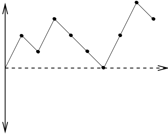
Figure 11: a generalized Dyck path of length nine with E = \{(1, 2), (1, -1)\}
