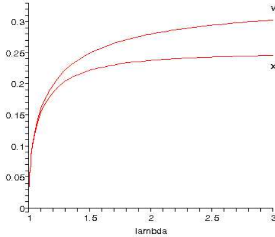
Figure 5: x and v plotted against \lambda
