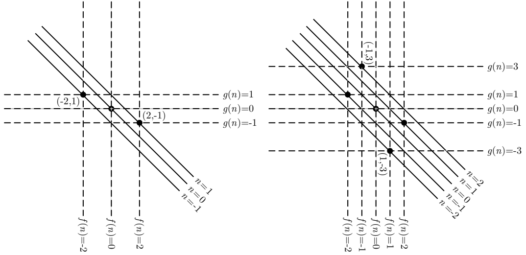
Figure 2: Evolving point selection.
