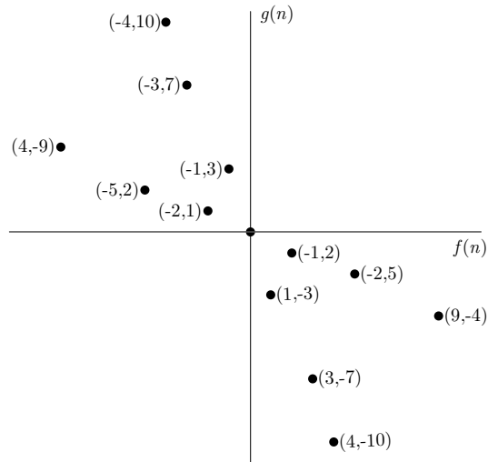
Figure 3: Plotted points up to n = \pm 6 .
