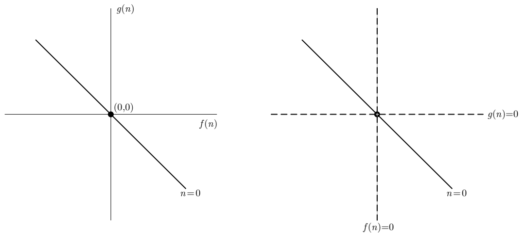
Figure 1: Beginning the point plot of f(n), g(n) in \mathbb{Z}^2 on the left. The first dashed keep off lines are shown on the right.
