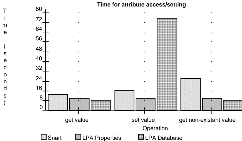
fig. B.10. Smart attribute access/assignment vs. Prolog database and LPA properties.
