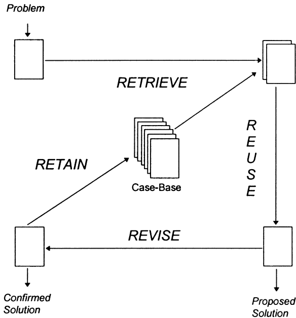
Fig. 1. The CBR-cycle after Aamodt and Plaza [6].
