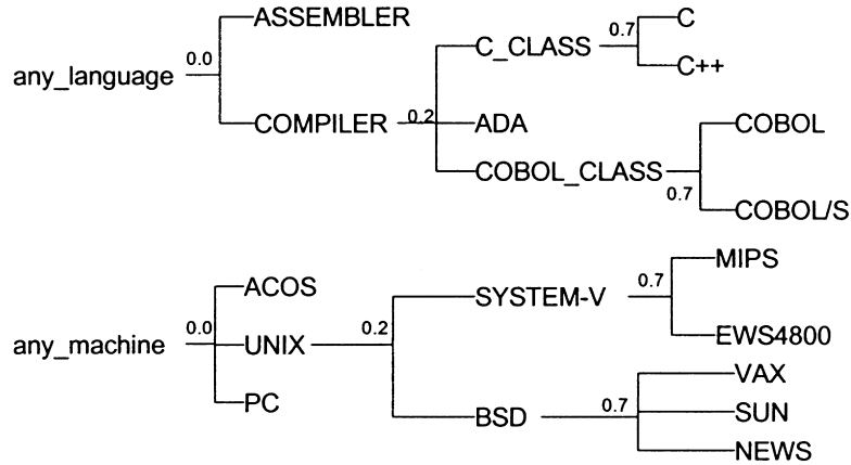
Fig. 4. Examples of abstraction hierarchies (after Kitano and Shimazu [14]).
