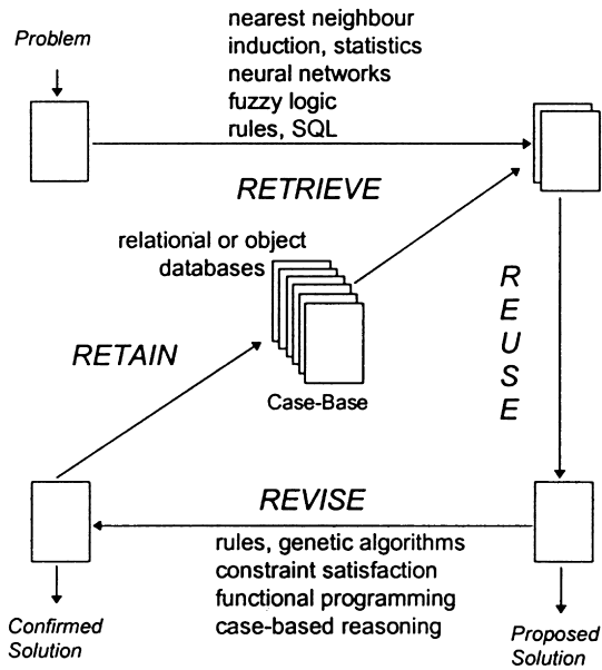
Fig. 5. Technologies and the CBR-cycle.
