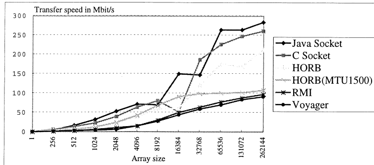
FIGURE 6. DOT Performance : byte array transfer with MTU = 9000
