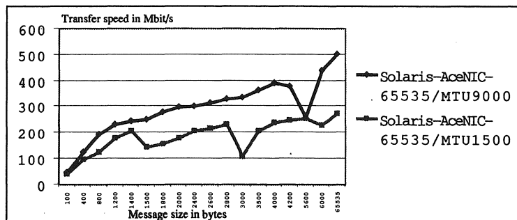
FIGURE 3. TCP/IP Performance with Netperf : MTU = 9000
