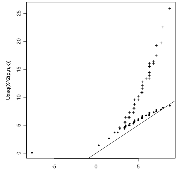
Umultinomial( n = 10, k = 100 ), accumulated in order of increasing X^2
