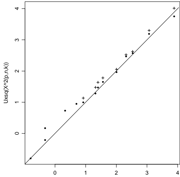
Umultinomial( n = 10, k = 3 ), accumulated in order of increasing X^2
