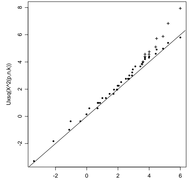
Umultinomial( n = 10, k = 10 ), accumulated in order of increasing X^2
