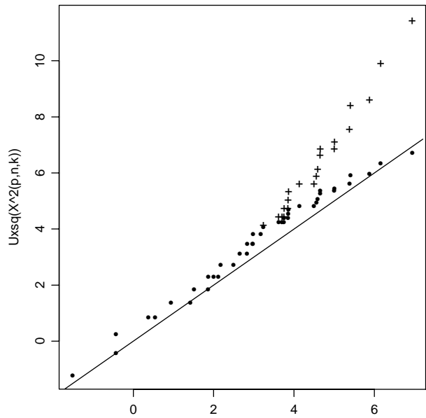
Umultinomial( n = 10, k = 20 ), accumulated in order of increasing X^2
