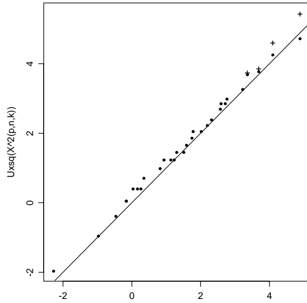
Umultinomial( n = 10, k = 5 ), accumulated in order of increasing X^2
