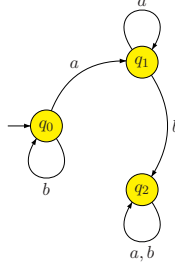
Fig. 1. The observed system is represented by the FSA \mathbb{A} = (\{q_0, q_1, q_2, a, b, :, \}, \{a, b\}, \delta, \{q_0\}) . For instance, the string aq_1ba : abq_2a denotes the transition from state q_1 to state q_2 reading the symbol b . A computation of \mathbb{A} is described by a sequence of strings over the alphabet of \mathbb{A} .
