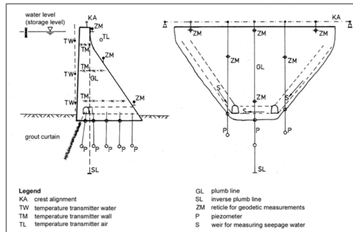
Figure 1 Example for the configuration of measuring devices [1]
