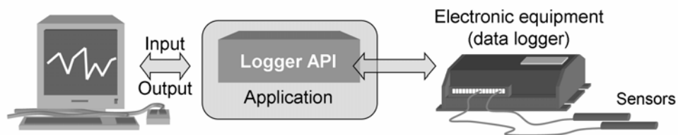
Figure 4 Control of a data logger via the Logger API
