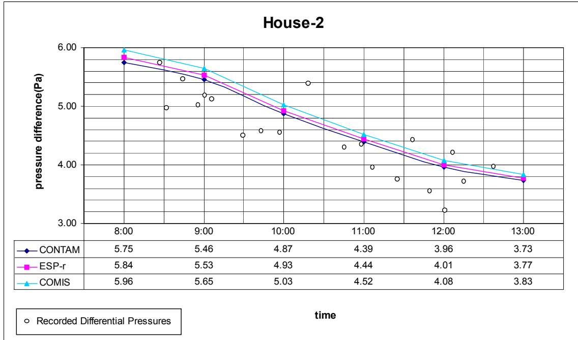
Figure 2 Measured and Predicted Differential Pressure across Garage-House Interface of House #2
