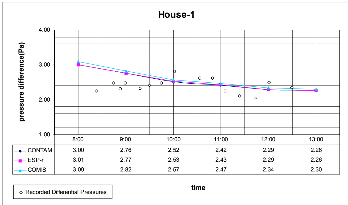
Figure 1 Measured and Predicted Differential Pressure across Garage-House Interface of House #1
