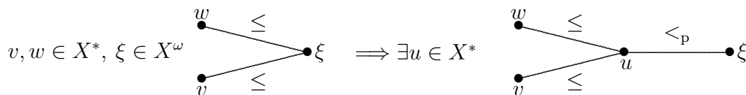
Fig. 2. The situation of Definition 14.
