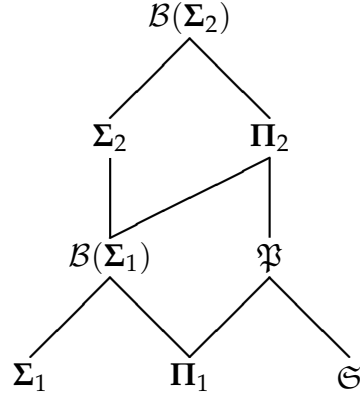
Figure 2: Inclusion relations between various classes of \omega -languages ( \mathcal{B}(\mathbf{K}) denotes the closure of \mathbf{K} under Boolean operations)
