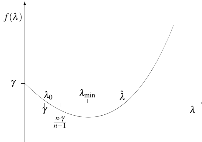
Figure 1: Plot of the function f(\lambda) in the case of two positive roots
