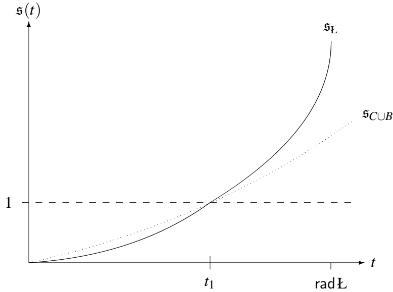
Figure 2: A typical plot of the structure generating functions of L and C \cup B
