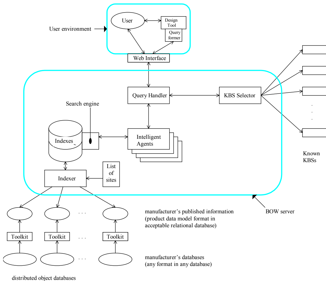
fig 1: BOW Architecture
