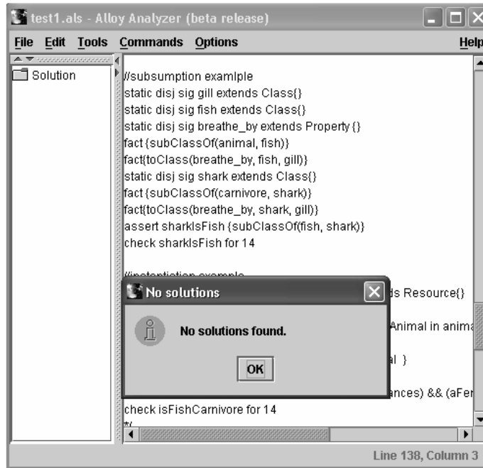
Fig. 3. Subsumption example.
