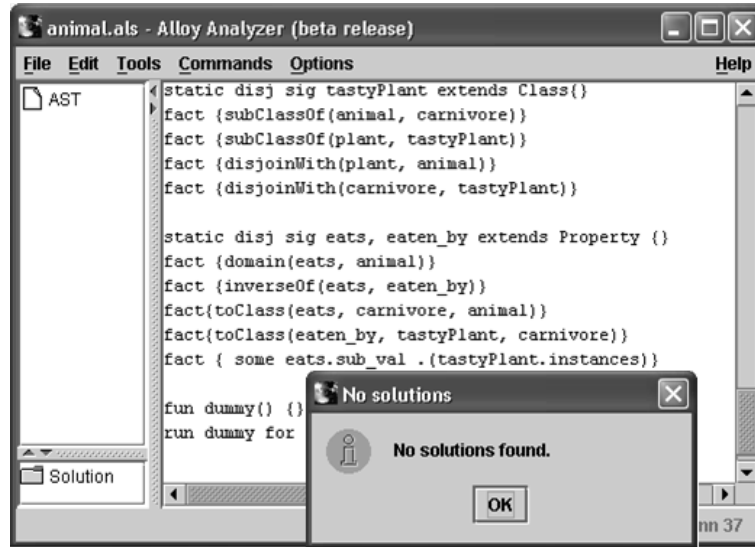
Fig. 1. Inconsistence example.
