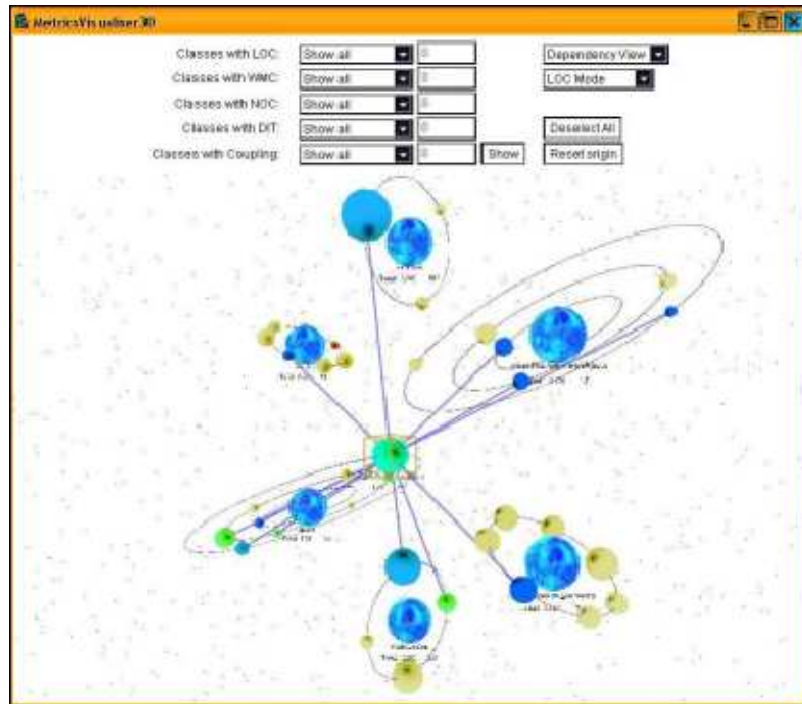
Figure 4: A screenshot of the solar system metaphor as applied to the source code of the tool itself. The true colour scheme is a real starscape, but colours have been inverted for clarity in publication.
