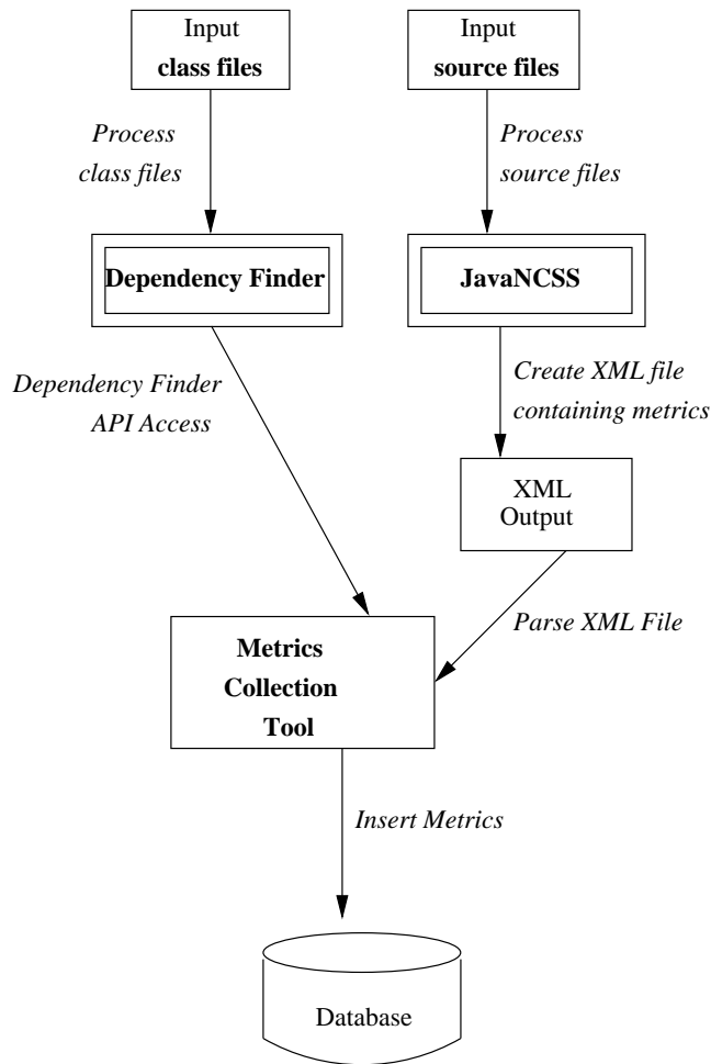
Figure 1: Metric collection system architecture for our study.
