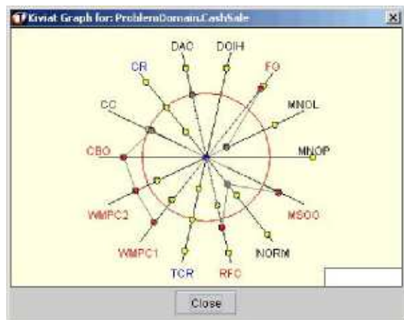
Figure 2: Kiviati charting as seen in the Borland's TogetherJ ( TogetherJ 2003)
