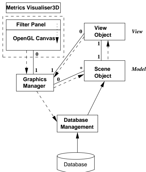
Figure 7: Underlying architecture of the 3D visualisation tool.
