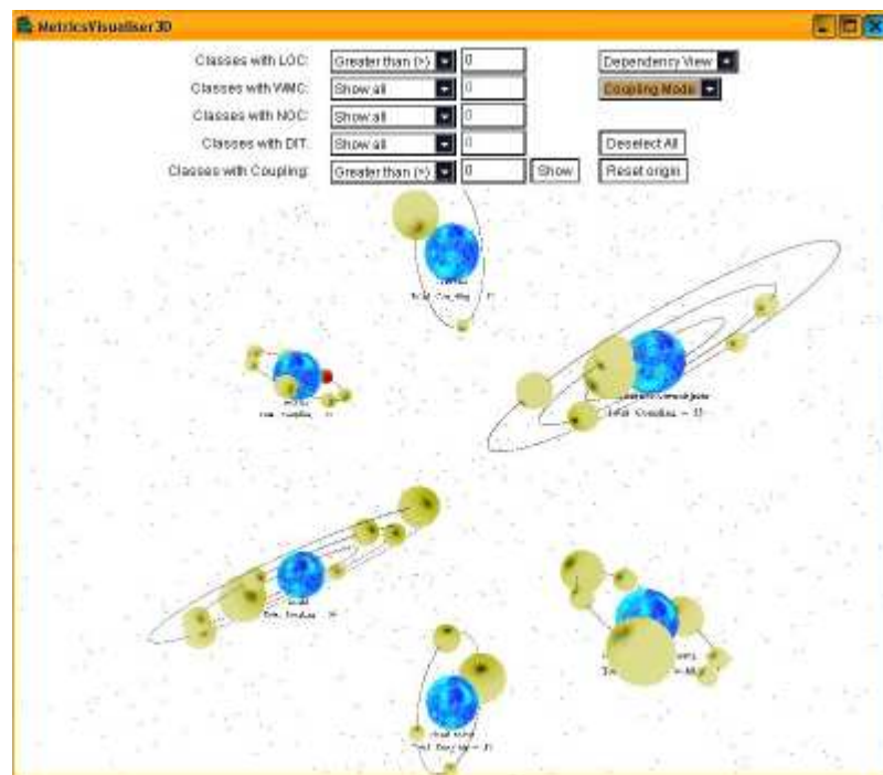
Figure 6: Visualisation in 'Coupling Mode'. Note the contrast in relative size of the planets in some orbits.
