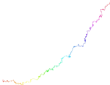
(e) A million step walk on EB(2) base 4 (normal?)
