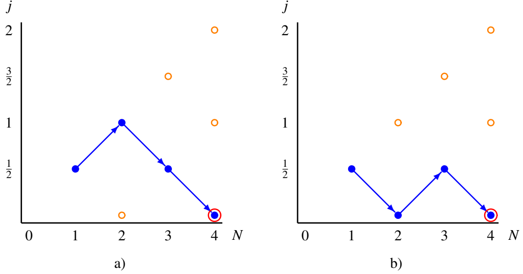
FIG. 7 Construction of both singlet states a) |\Psi_{2,4,1}\rangle of Eq. (54) and b) |\Psi_{2,4,2}\rangle of Eq. (55) of four spin- \frac{1}{2} particles. Concentric circles indicate the target states. The second state is a “zigzag” state composed by the product of two two-partite singlet states. The two-dimensional diagram represents the “space” or “domain” of all multi-partite states, whereby the number of particles is represented by the abscissa (the x -coordinate) along the positive x -axis. The ordinate (the y -coordinate) of the state is equal the total angular momentum of the state. Note that a single point may represent many states; all corresponding to an equal number of particles, and all having the same total angular momentum. N -partite singlet states can be constructed by starting from the unique state of one particle, then proceeding via all “diagonal” and, whenever possible for integer spins, also “horizontal” pathways consisting of single substeps adding one particle after the other — either diagonally from the lower left to the upper right “↗,” or diagonally from the upper left to the lower right “↘,” or, if possible, also horizontally from left to right “→” — towards the zero momentum state of N particles. Every diagonal or horizontal substep corresponds to the addition of a single particle.
