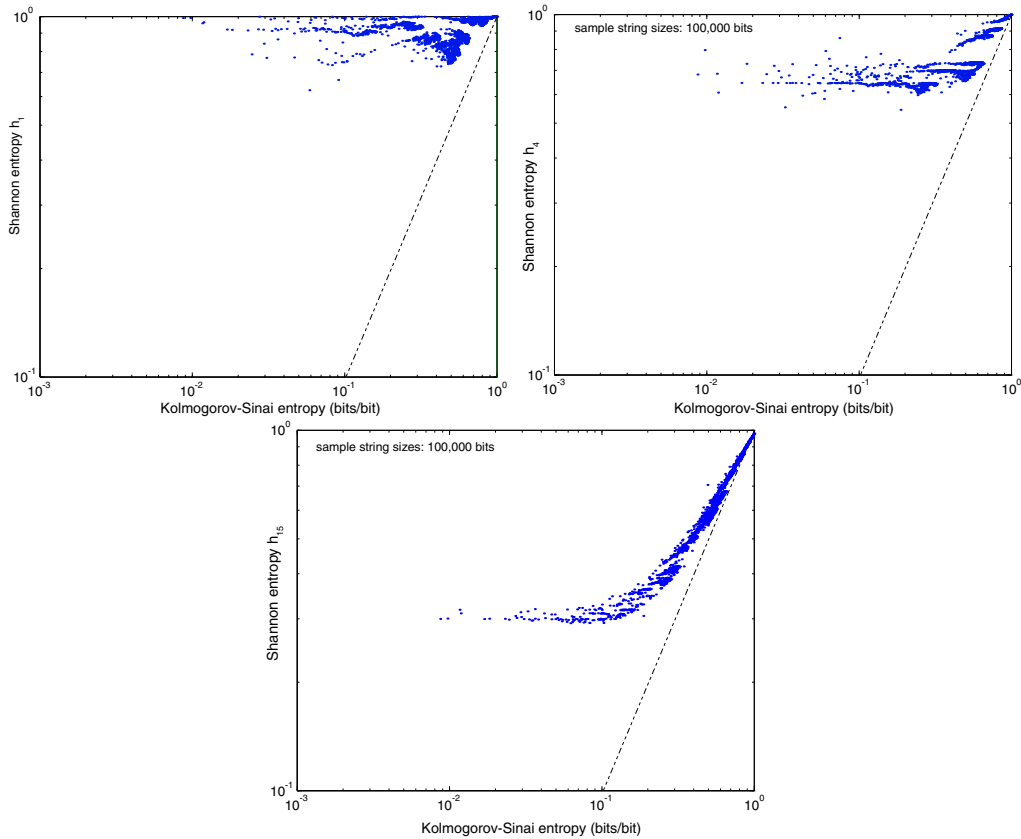
Fig. 1. Shannon n -block entropies for n = 1, 4, and 15, for sample strings produced from the logistic map.
