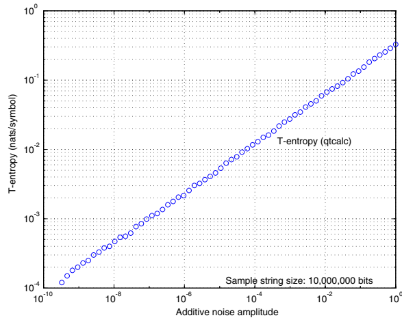
Fig. 7. T-entropy as a function of additive noise amplitude.
