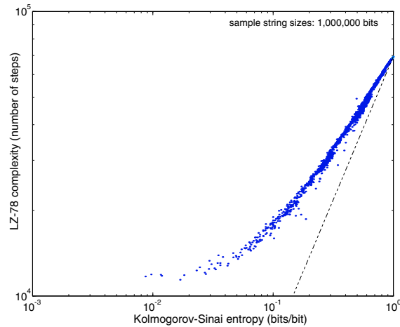
Fig. 3. LZ-78 complexities versus corresponding KS-entropy values.
