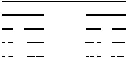
FIG. 1: First construction steps of a generalized Cantor set.
