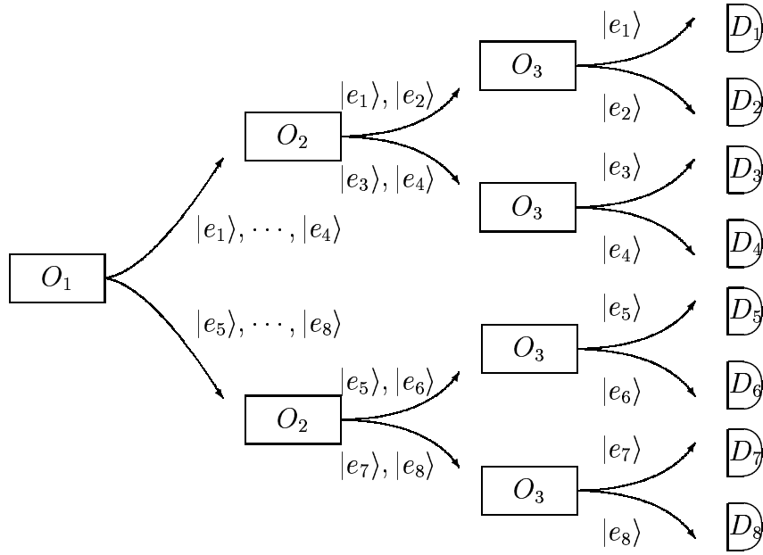
FIG. 1: State sieve resulting from binary search. Successive measurements of propositions O_1, O_2, O_3 serve as filters to single out the input state. D_1, \dots, D_8 indicate the final detectors; In the lossless case, exactly one of them clicks.
