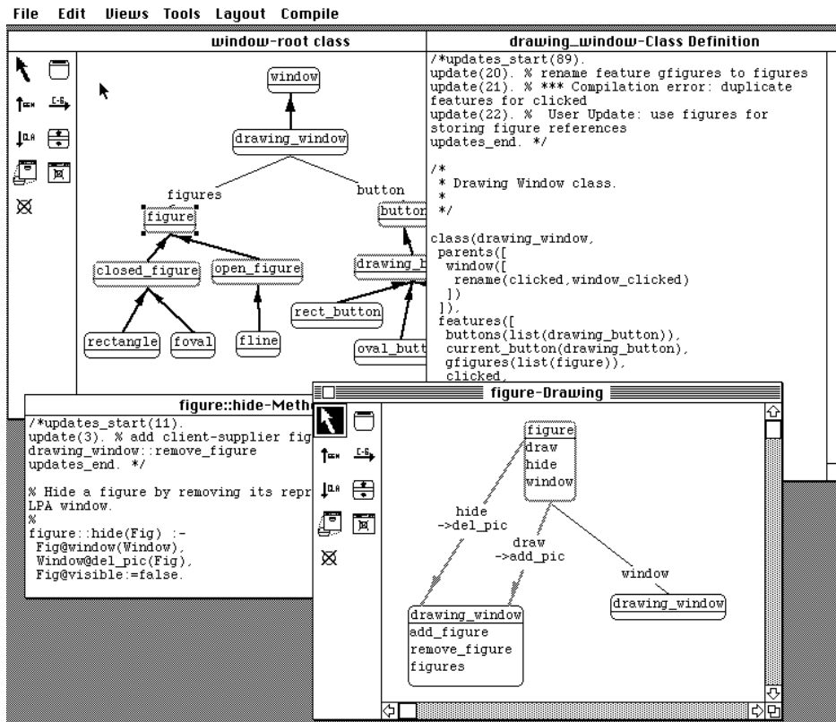
Figure 1. The Smart Programming Environment.
