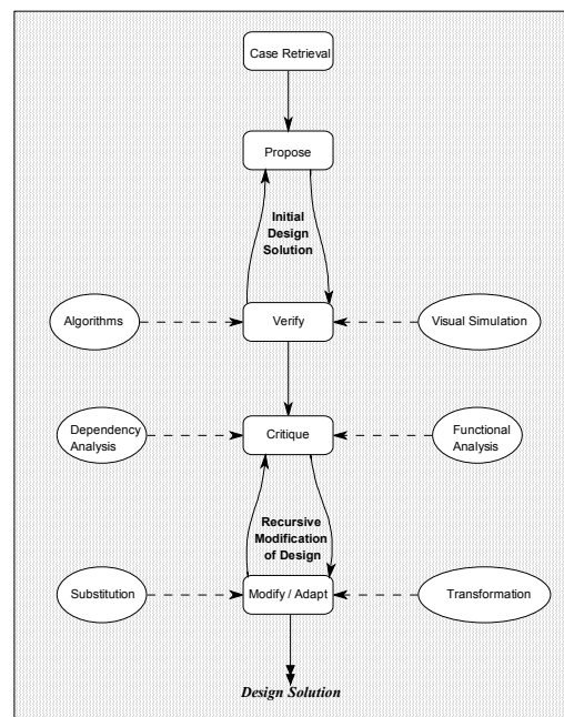
Figure 3 Overview of PCM Method for Design
