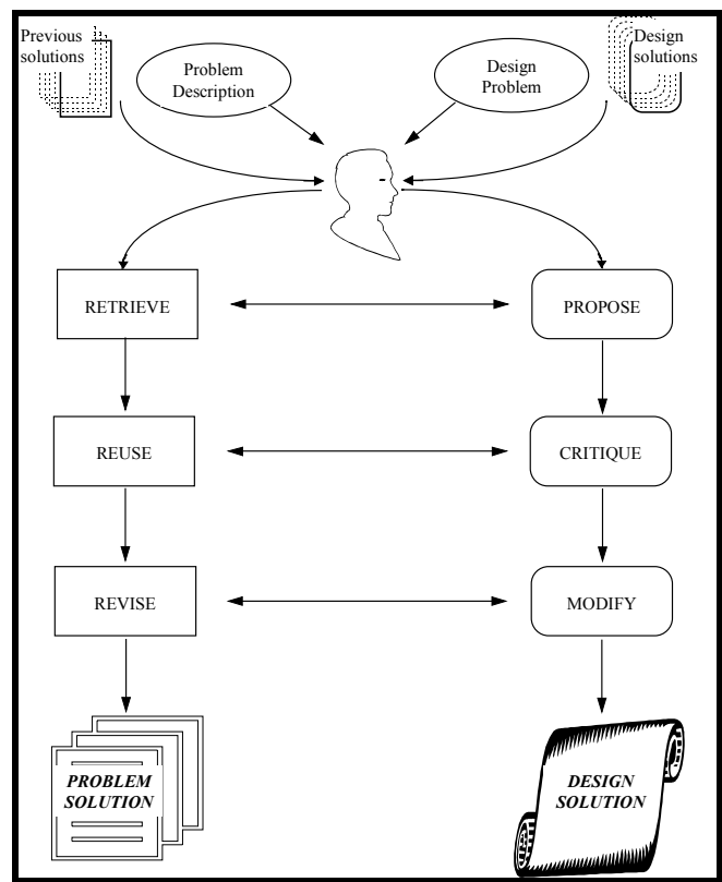
Figure 4 Mapping The Design Task to the CBR-cycle
