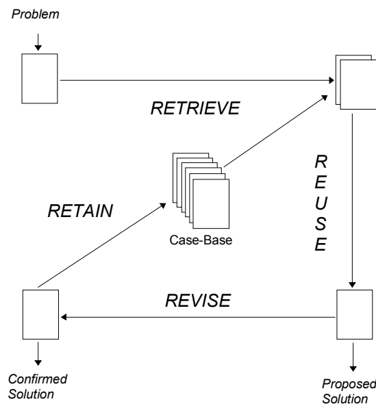
Figure 1 The CBR Cycle
