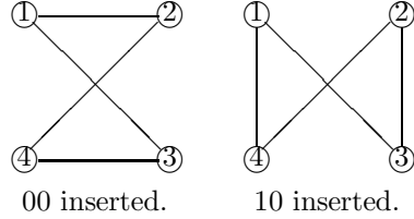
Figure 4.3: The interference graphs for watermarked programs recognized as TRUE
