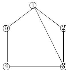
Figure 3.3: The result interference graph by inserting one bit “0”
