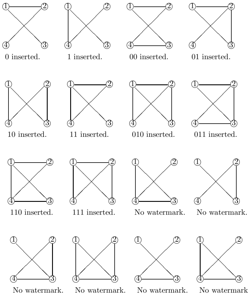
Figure 4.1: The interference graphs for watermarked programs recognized as TRUE
