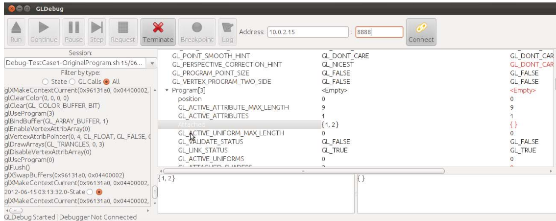
Figure 2: The GLDebug interface comparing two sets of captured state.
