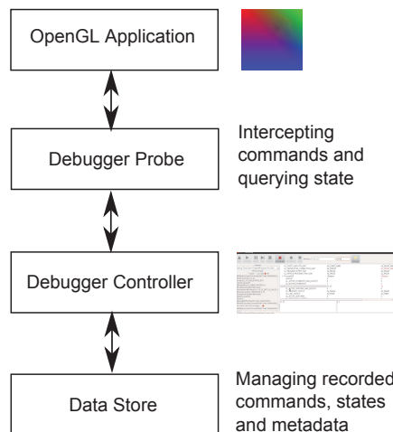
Figure 1: Architectural overview of GLDebug.
