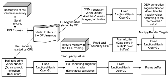
Figure 8: Overview of the first rendering algorithm.
